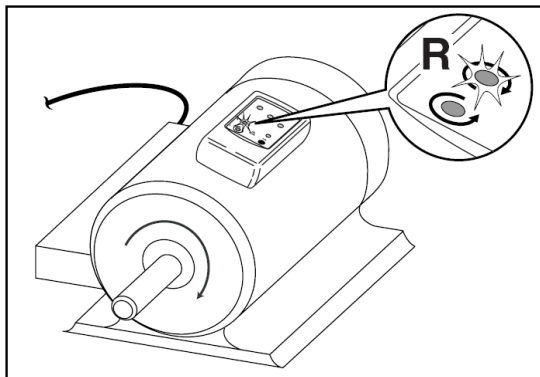
Figure 3. Motor Rotation
