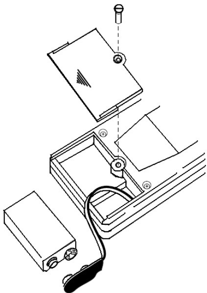
Figure 4. Battery Replacement
